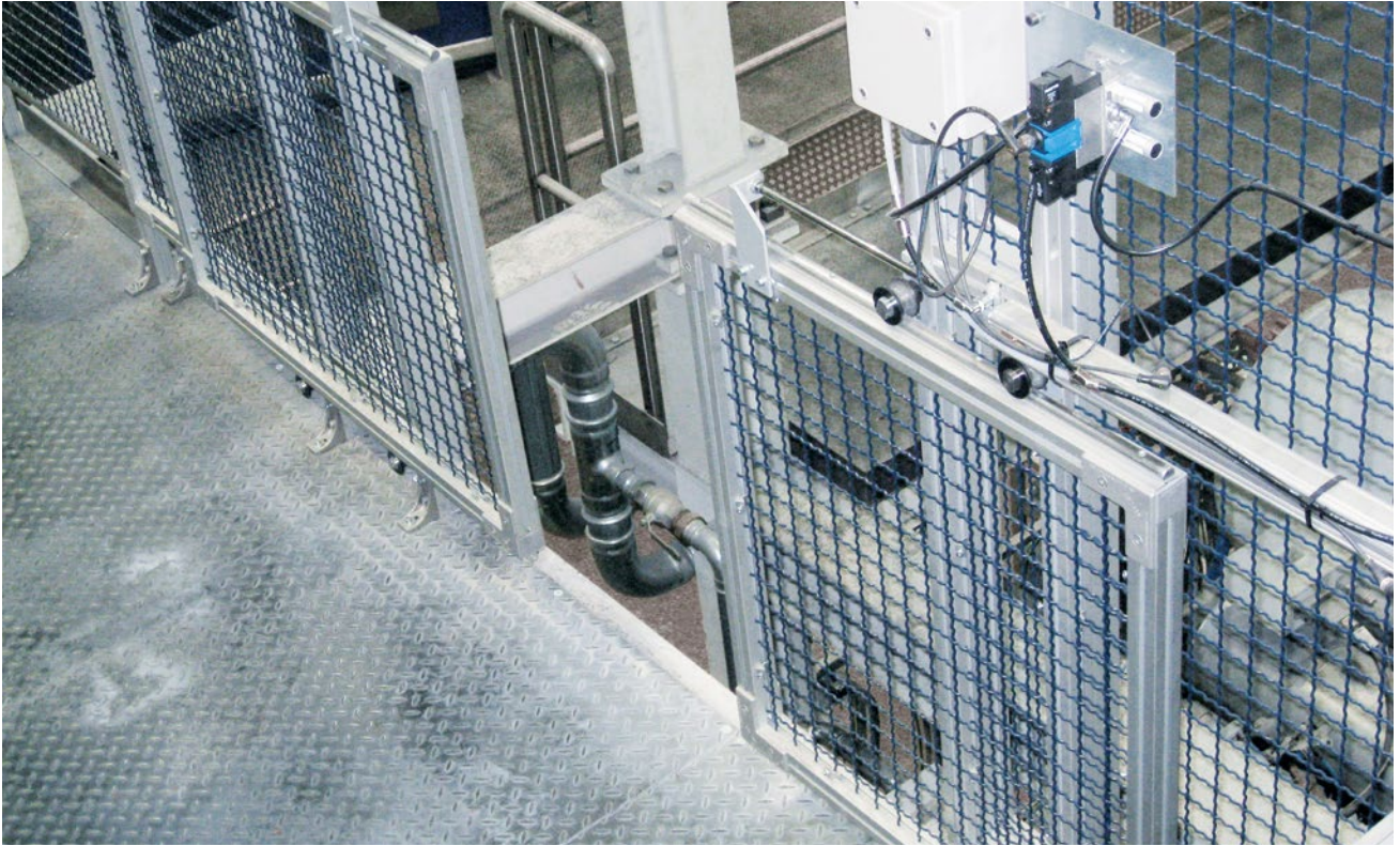
Double sliding gate
